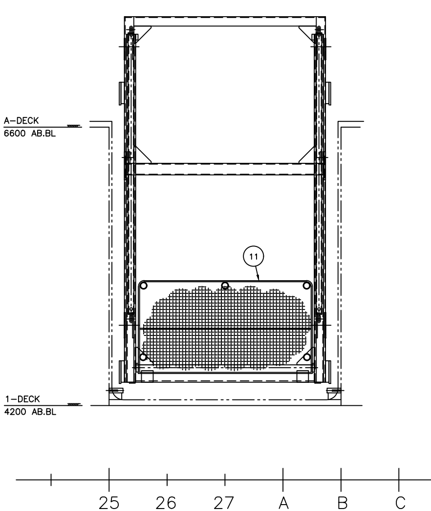
SIDE VIEW OF PLATFORM STOWED POSITION SHOWN LOOKING PORT
