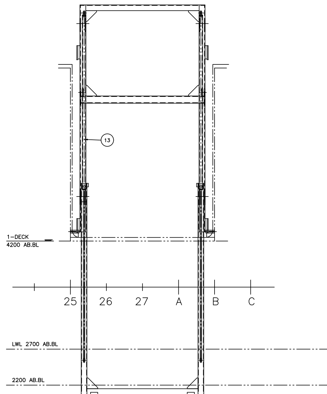
SIDE VIEW OF PLATFORM LAUNCHED POSITION SHOWN LOOKING PORT
