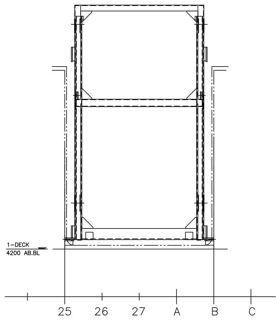
SIDE VIEW OF PLATFORM LAUNCHED POSITION SHOWN LOOKING PORT
