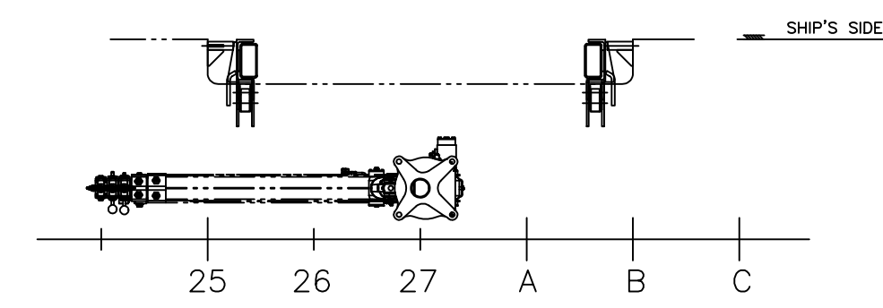
PLAN VIEW OF PLATFORM SECTION AT A-DECK STOWED POSITION SHOWN
