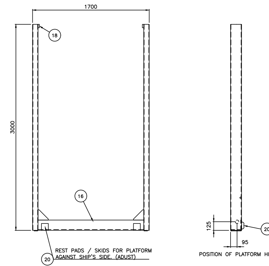
MOVABLE PLATFORM FRAME
