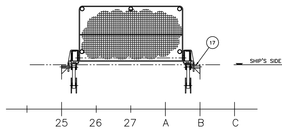
PLAN VIEW OF PLATFORM SECTION AT 1-DECK LAUNCHED POSITION SHOWN
